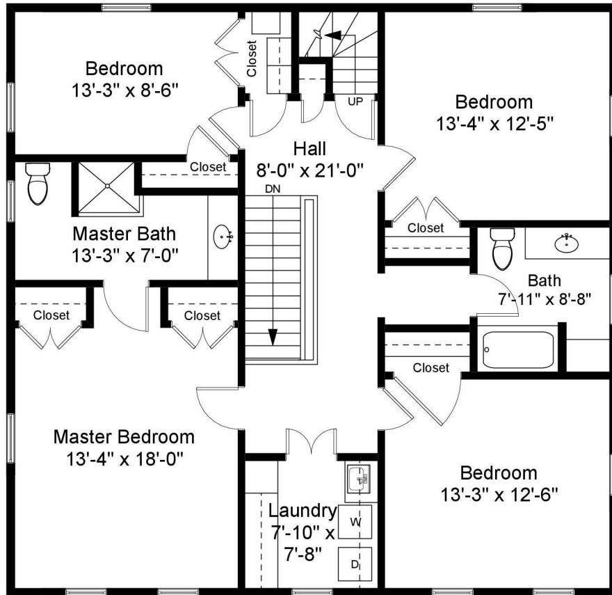
Second Floor Plan Ceiling Height = 8'-10"
