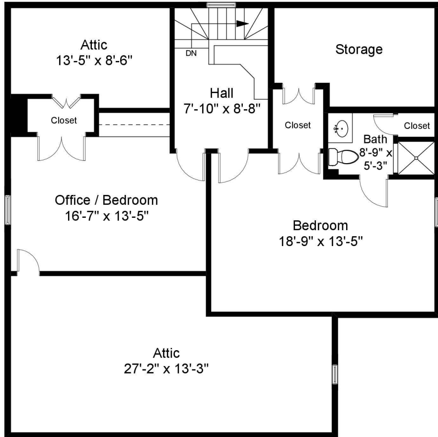
Third Floor Plan Ceiling Height = 7'-10"
